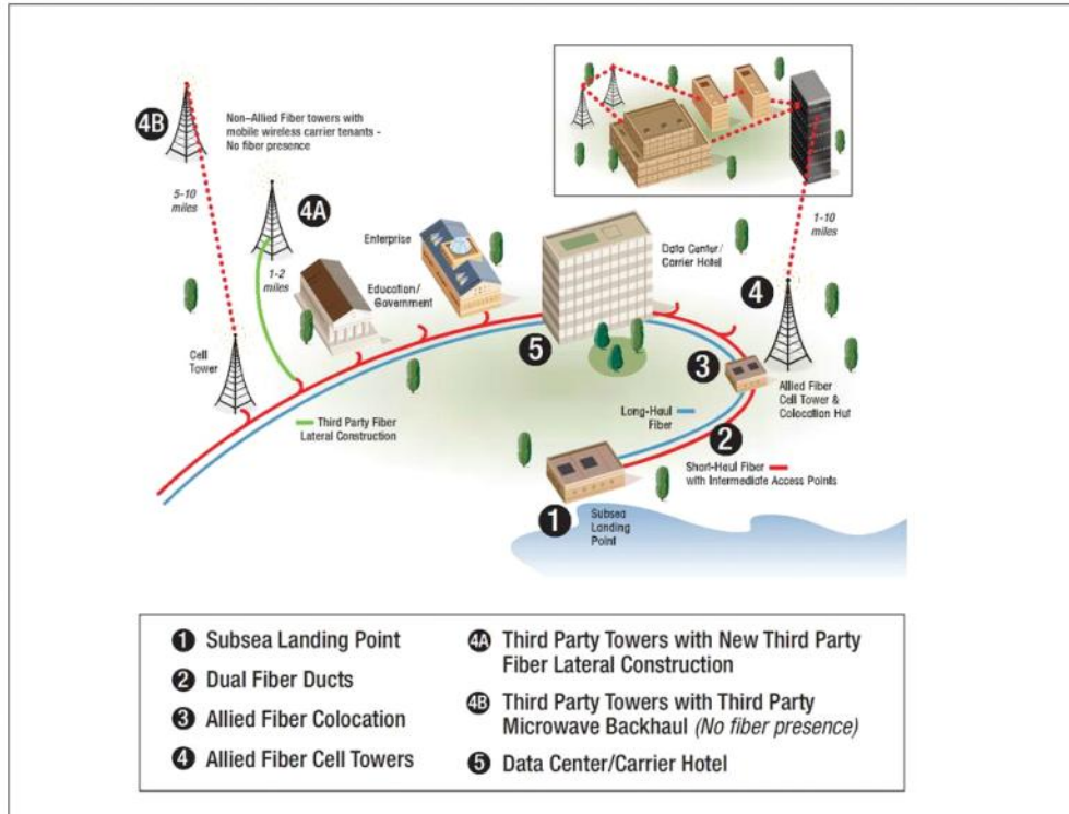
Figure 1. The multiduct system starts at the point of origin — the location where international cables come up from the ocean, also known as subsea landing points.
